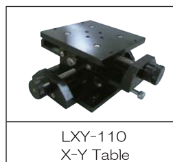
LXY-110 X-Y Table Max. load 500 N Moving distance X = 75mm Y = 75mm
