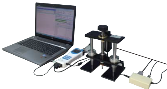
Temperature expansion coefficient evaluation for load application device
