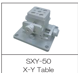
SXY-50 X-Y Table Max. load 500 N Moving distance X = 30mm Y = 30mm
