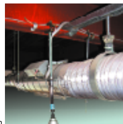
Hanger bolts for duct installation
